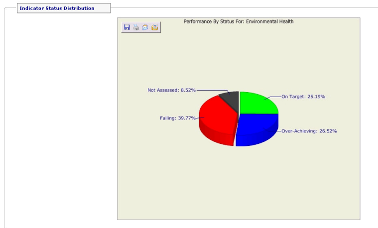
Figure 2: Performance drill-down
